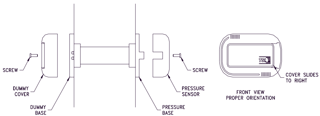
Figure 4: Pressure Sensor Mounting
