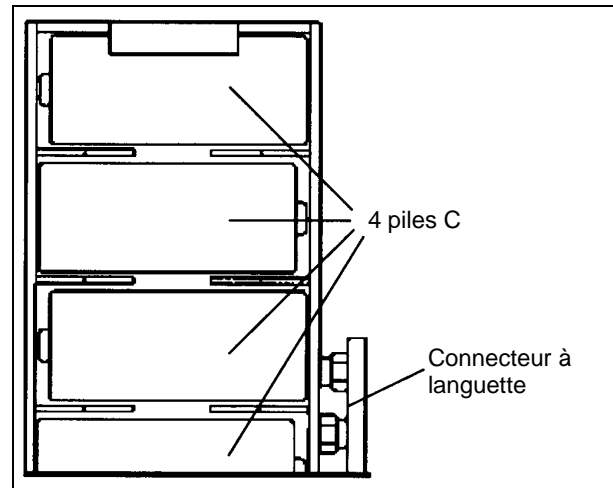
Figure 2 Porte-piles
