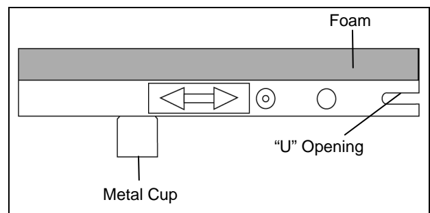
Figure 1 Hood Frame Channel
