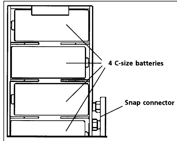
Figure 2 Battery Holder
